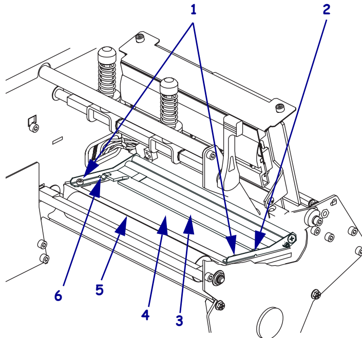
Figure 28 • Snap Plate for R110Xi/R170Xi and RFID-Ready XIIIPlus Printers
