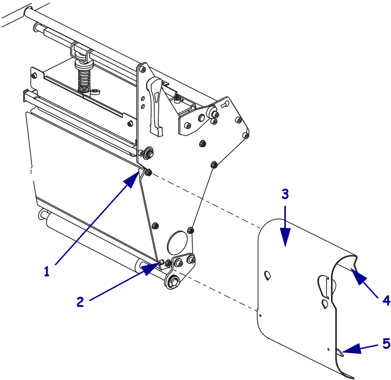
Figure 23 • Rewind Plate
