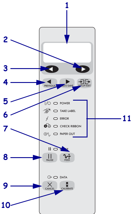
Figure 4 • Location of Control Panel Buttons and Lights
