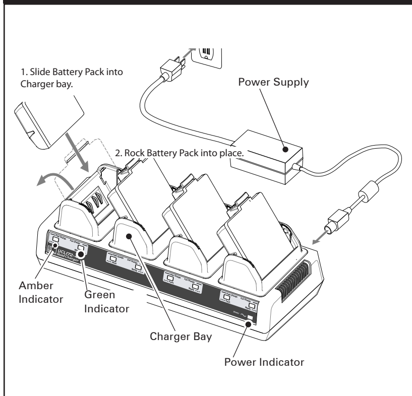
Figure 5: Quad Charger
