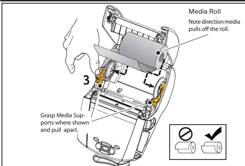
Figure 12: Loading Media
