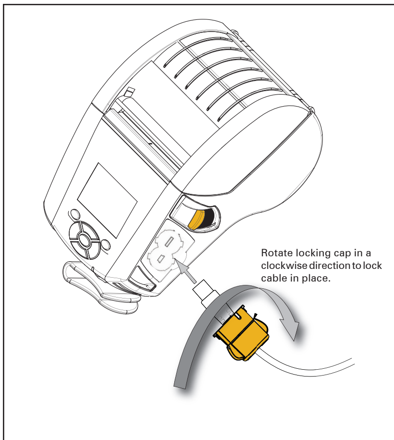
Figure 20: Communications Port Strain Relief
