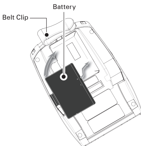
Figure 2: Installing the Battery
