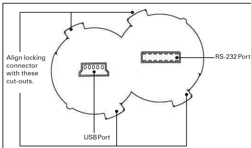
Figure 19: Communications Port
