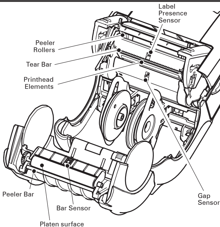
Figure 22: Cleaning the QL 220 Plus
