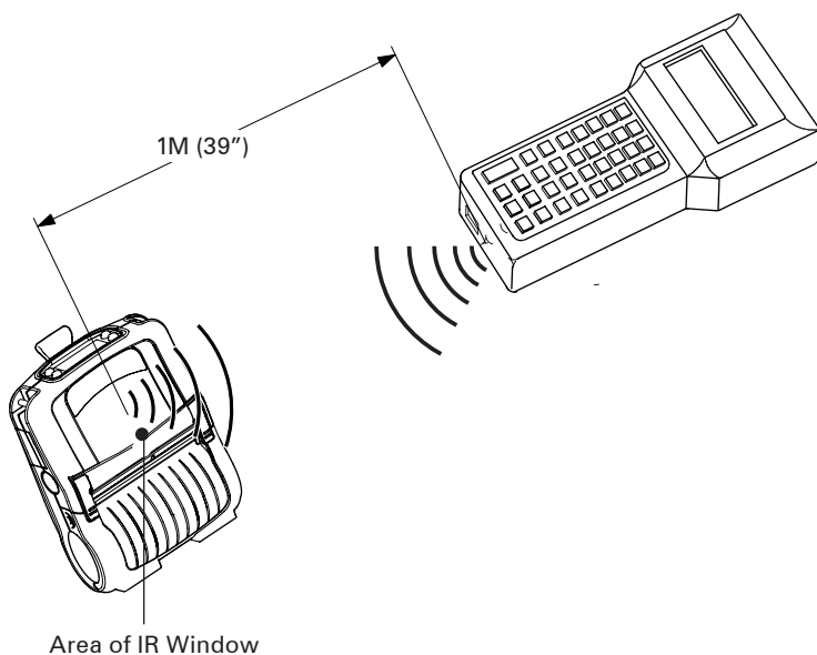
Figure 16: IR Communications
