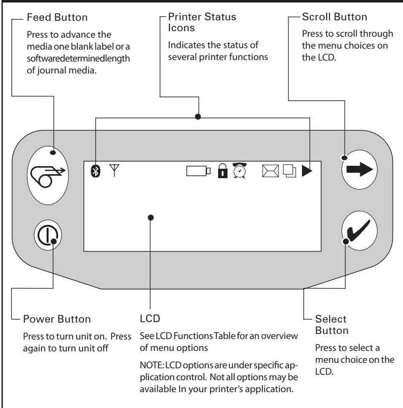
Figure 11: Optional LCD Control Panel
