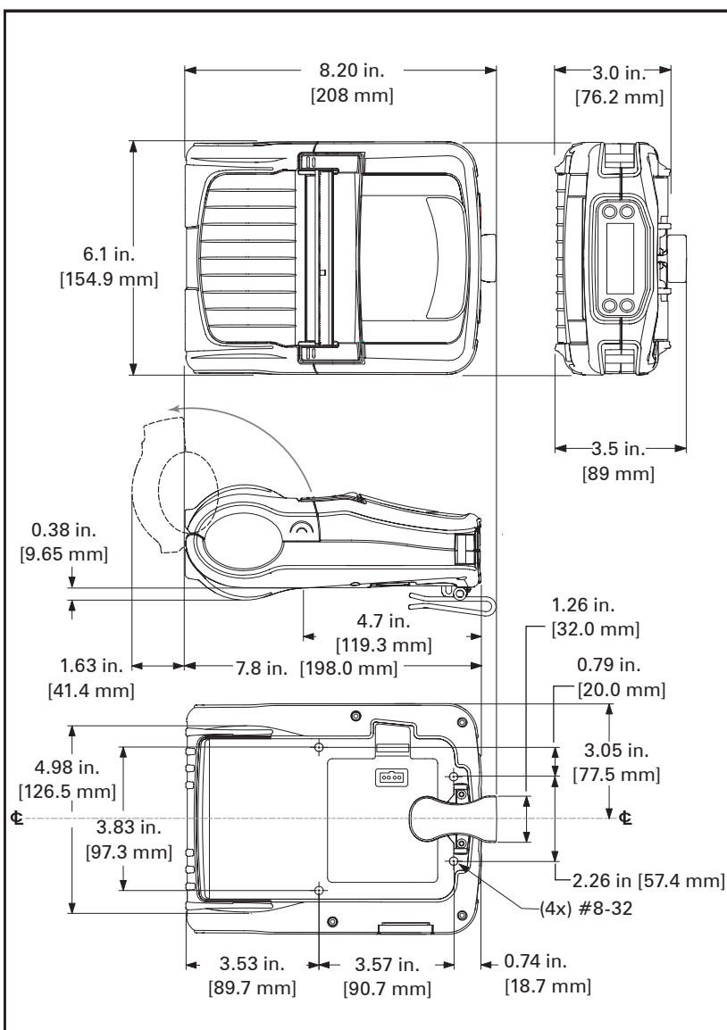
Figure 31: QL 420 Plus Overall Dimensions
