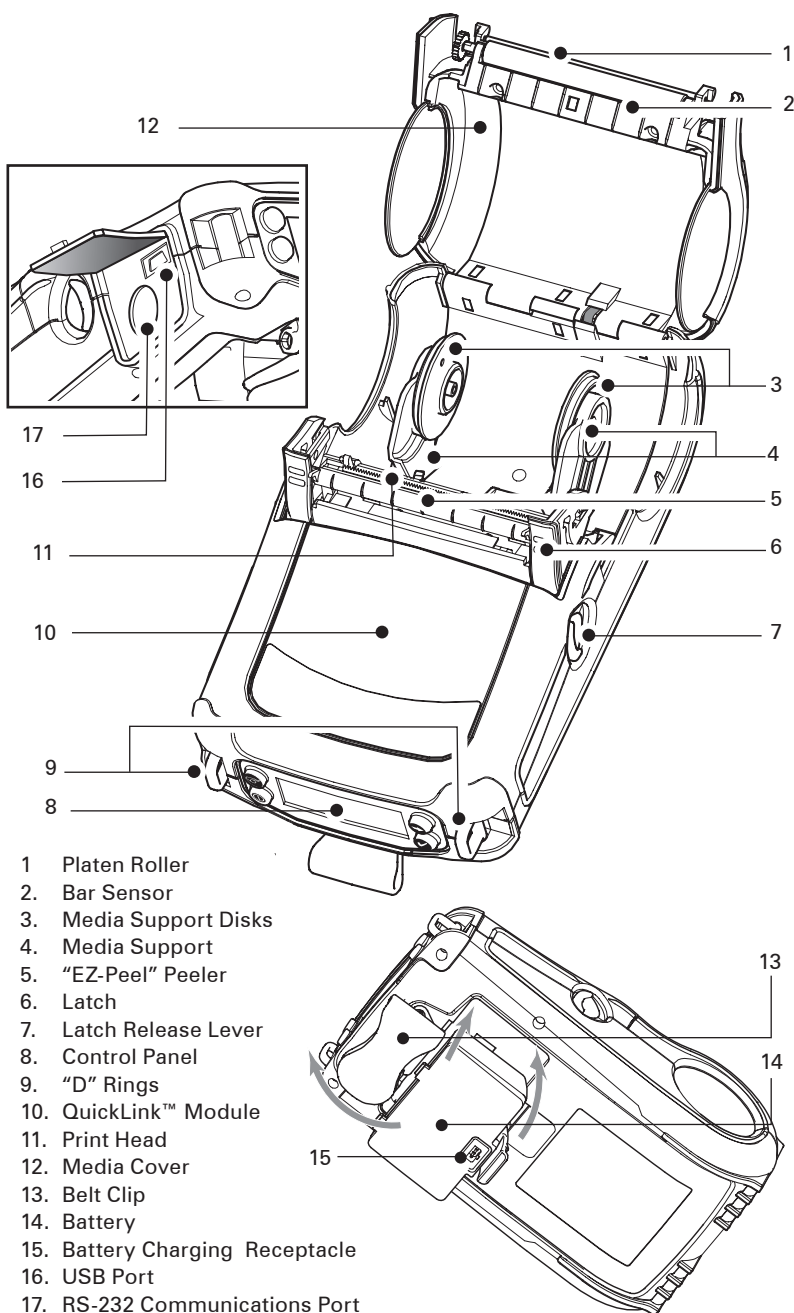
Figure 1B: QL 320 Plus
