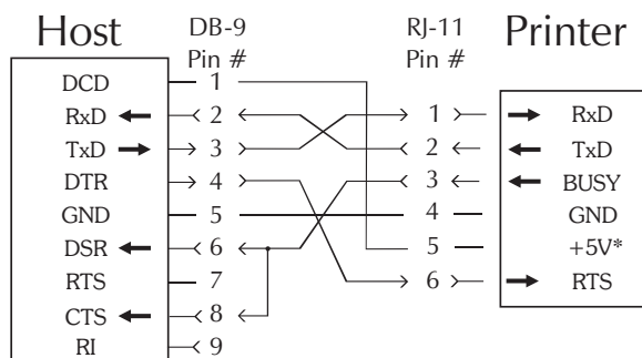
Female DB-9 to RJ-11
